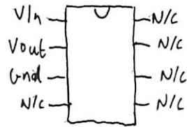
SG3503 2.5V Reference
